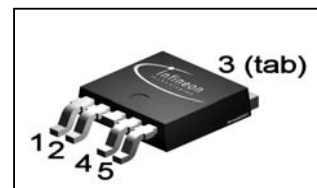
PG-TO252-5-3
